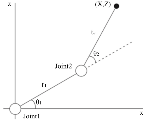
Figure 3. 2 link arm.
